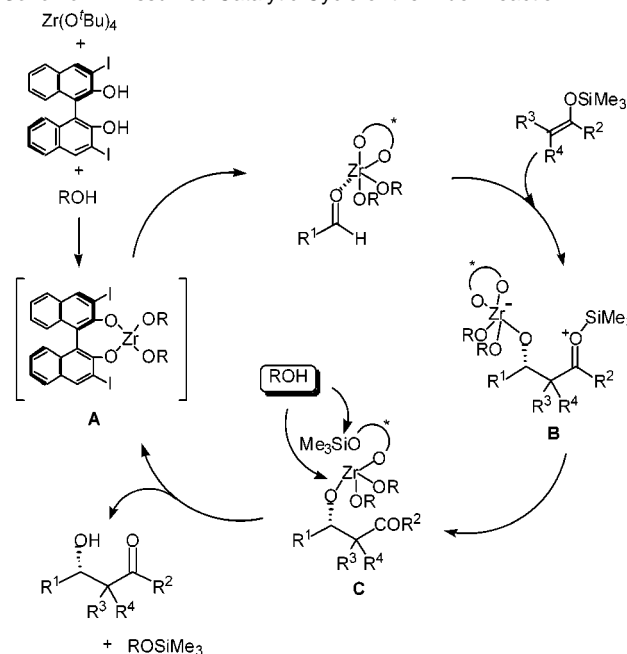
Figure 6. Assumed transition states for the anti -selectivity.
