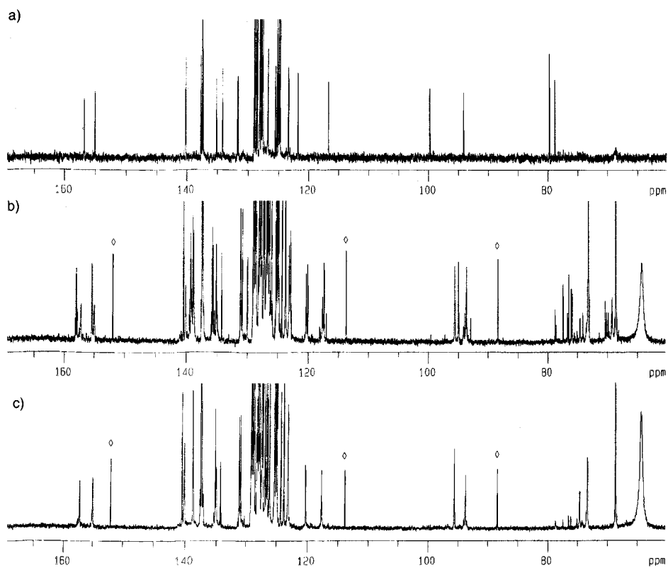
Figure 1. 1 H and 13 C NMR spectra of the zirconium complex. a
